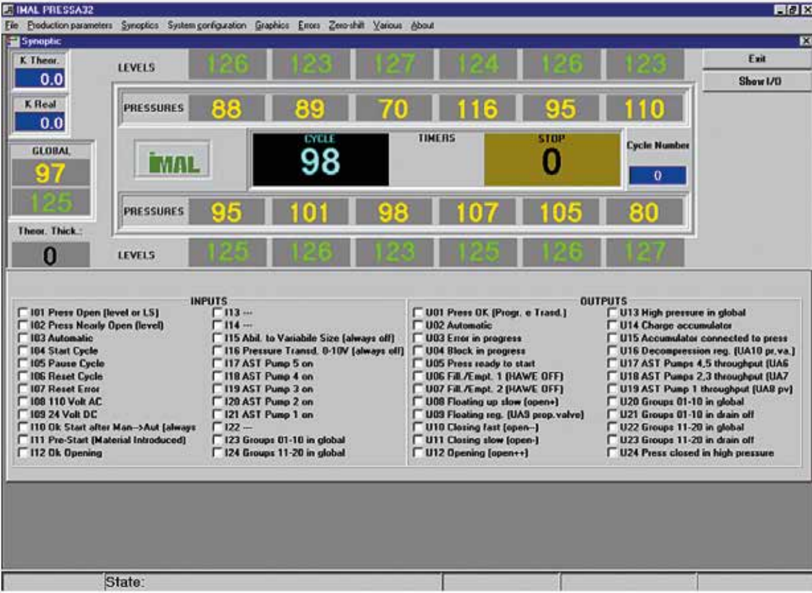
CHART SHOWING PRESSURE AND LEVEL VALUES FOR EACH PRESS CYLINDER
